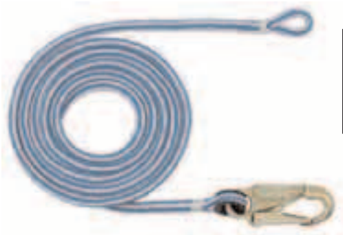
FL-1601 Non-Wire Core 16-strand Polyester double braid. Hand-spliced thimble eye and double-locking forged steel safety snap.
